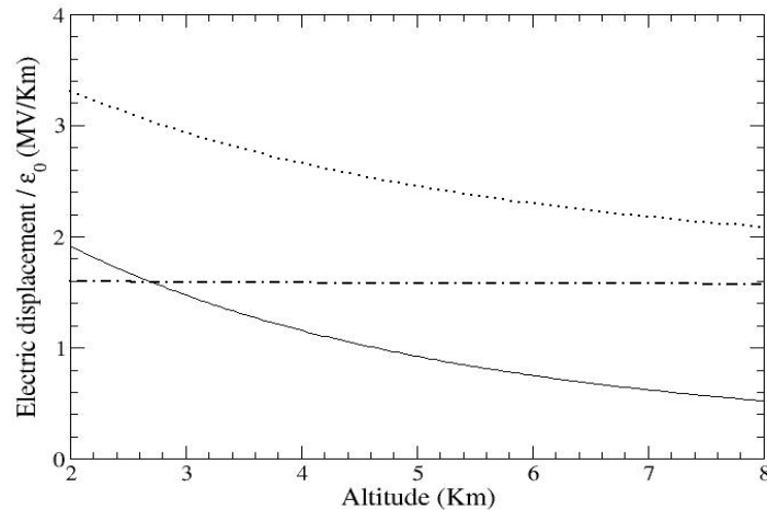
Figure 1: Contributions to the electrical displacement of the cloudy cell at different altitudes: water plus a fraction of methane (dotted line), only water (solid line), a methane fraction (dashed-dotted line).
