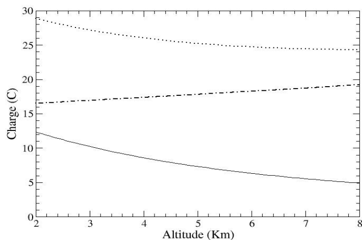
Figure 2: Maximum charge accumulated by the cloudy cell depending on the altitude of different components; water plus a fraction of methane (dotted line), a methane fraction (dashed-dotted line) and only water (solid line).
